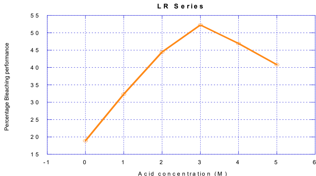
Fig. 3: Bleaching performance of LR sample
