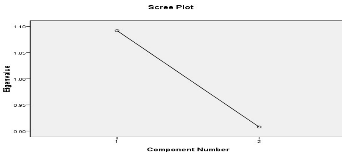
Figure 1: Scree plot for the component number analysis
