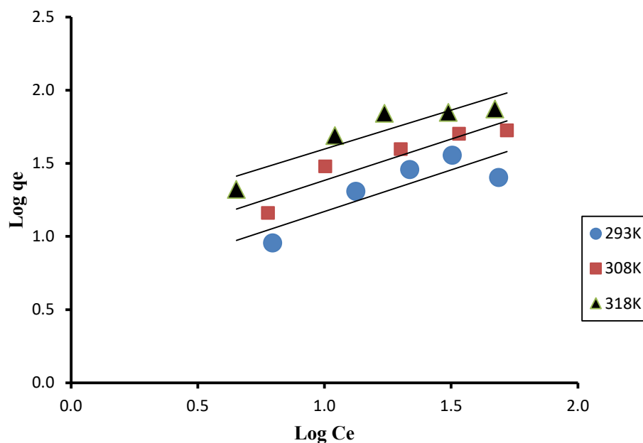
Fig.3 Freundlich isotherm at different temperature for Pb(II) ion adsorption onto Modified Chitosan (MC).
