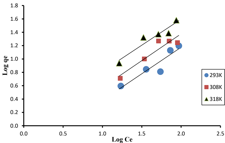
Fig.4 Freundlich isotherm at different temperature for Pb(II) ion adsorption onto Unmodified Chitosan (UC)
