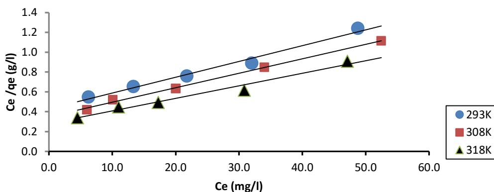
Fig.1 Langmuir isotherm at different temperature for Pb(II) ion adsorption onto Modified Chitosan (MC).
