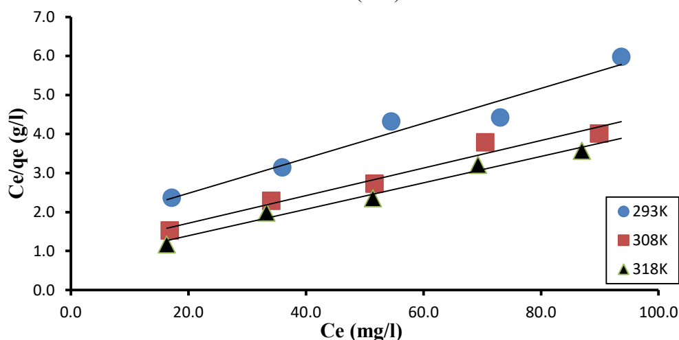
Fig.2 Langmuir isotherm at different temperature for Pb(II) ion adsorption onto Unmodified Chitosan (UC).
