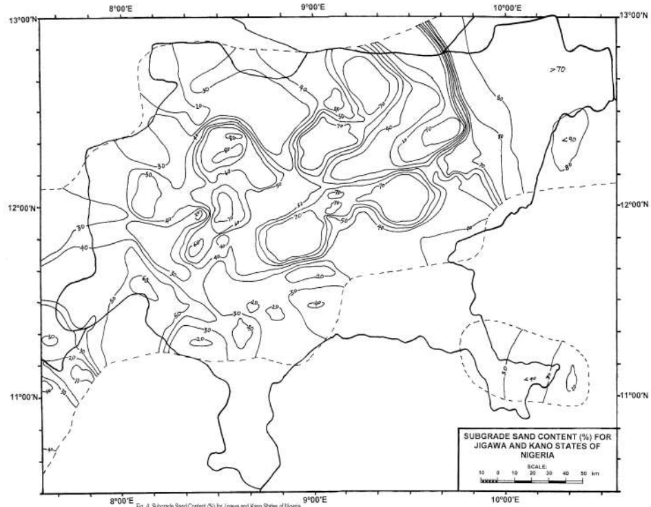
Fig. 4: Subgrade Sand Content (%) for Jigawa and Kano States of Nigeria
