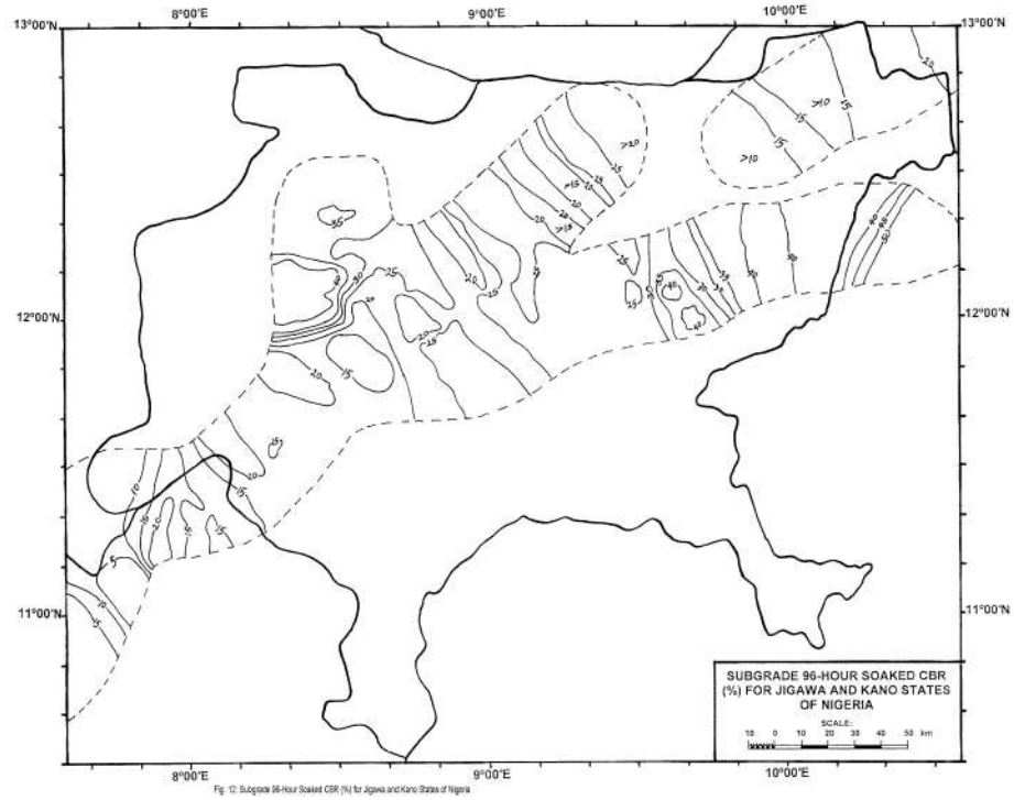
Fig. 12: Subgrade 96-Hour Soaked CBR (%) for Jigawa and Kano States of Nigeria
