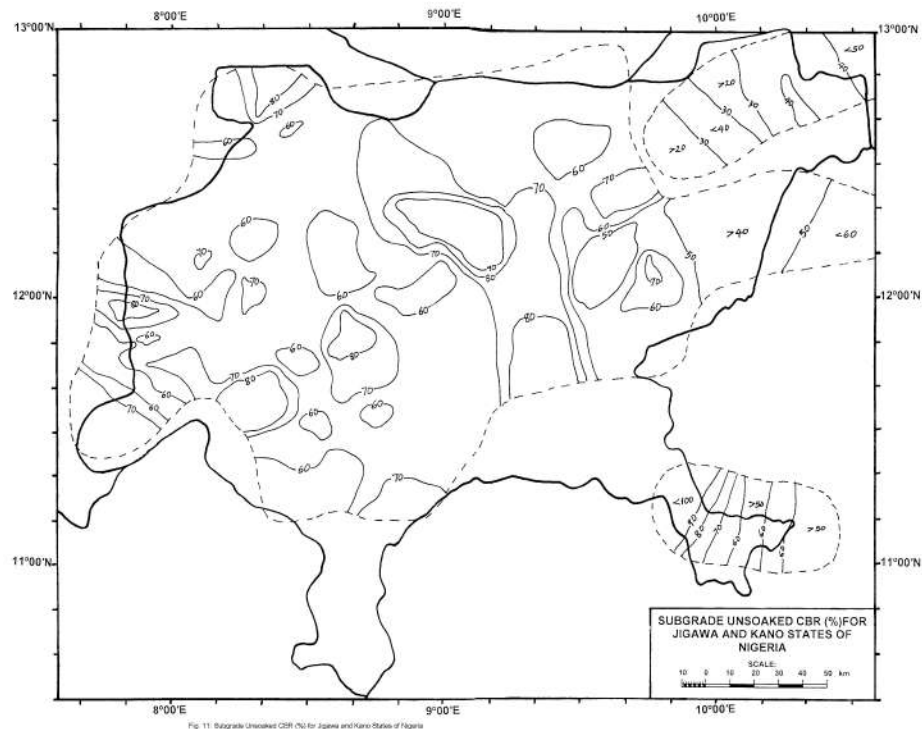
Fig. 11: Subgrade Unsoaked CBR (%) for Jigawa and Kano States of Nigeria
