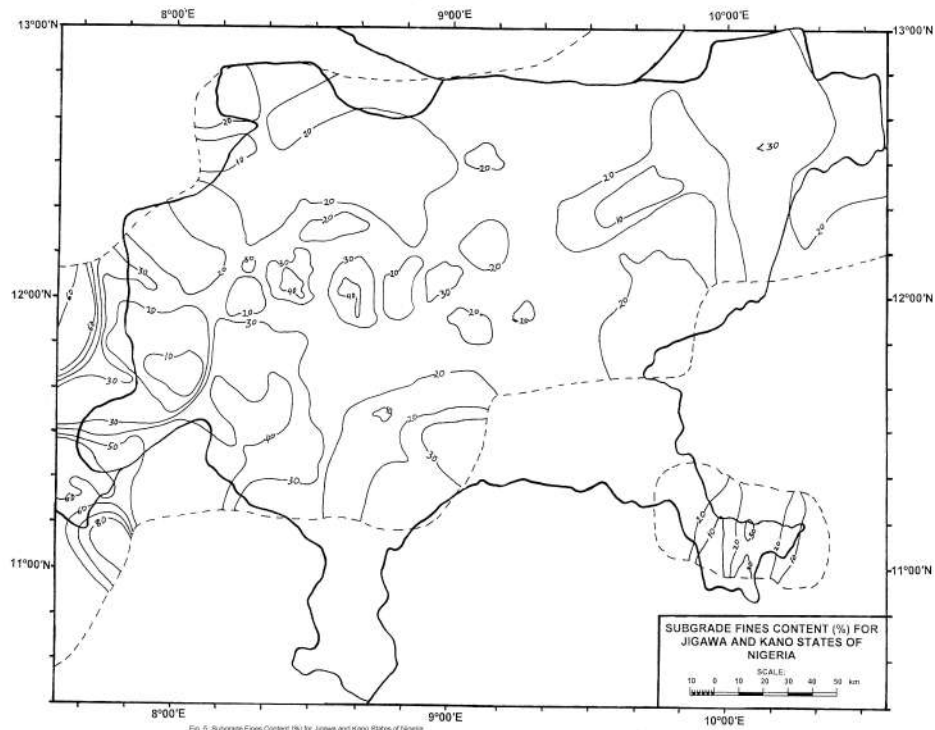
Fig. 5: Subgrade Fines Content (%) for Jigawa and Kano States of Nigeria
