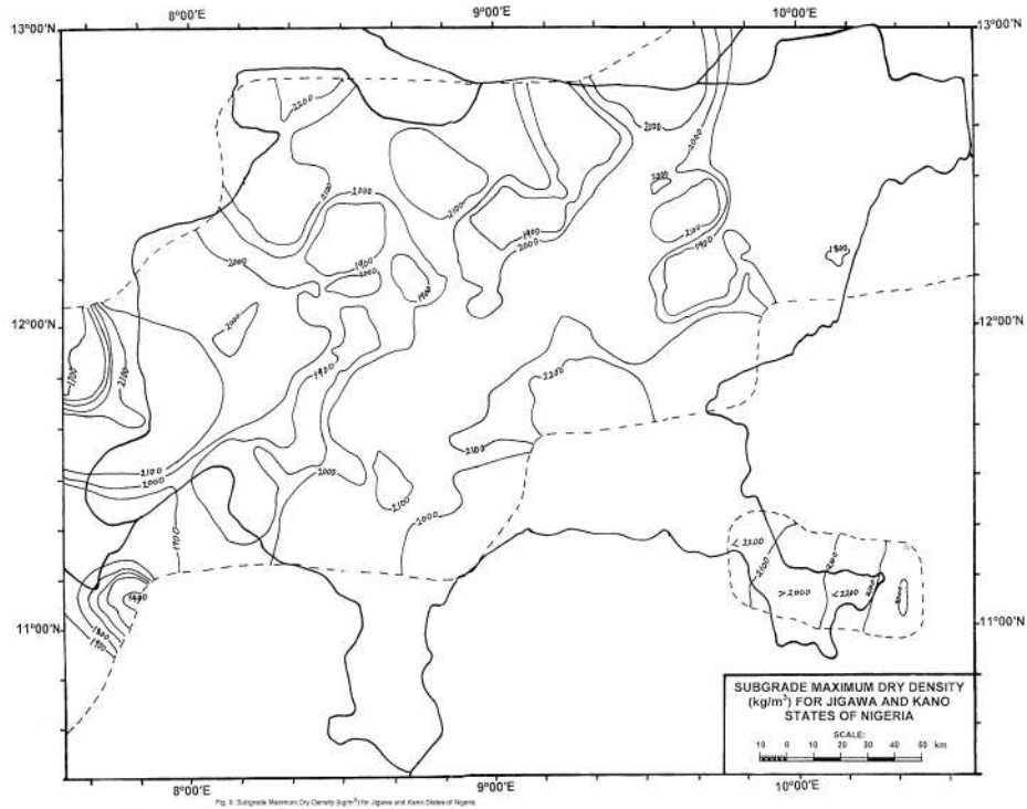
Fig. 9: Subgrade Maximum Dry Density (kg/m³) for Jigawa and Kano States of Nigeria
