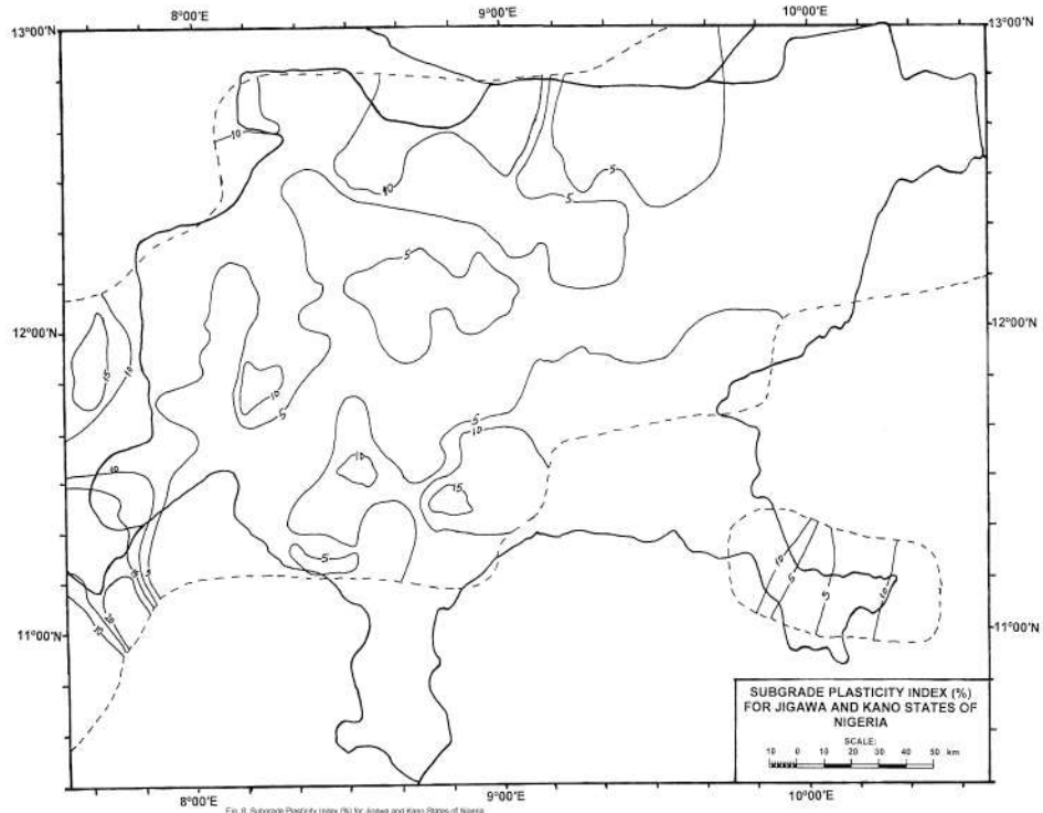
Fig. 8: Subgrade Plasticity Index (%) for Jigawa and Kano States of Nigeria
